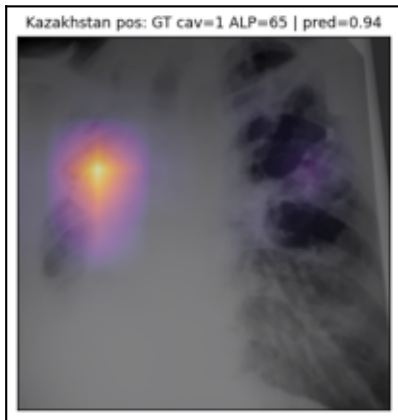
Kazakhstan cavity+: p=0.94
