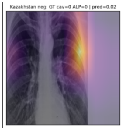
Kazakhstan cavity-: p=0.02
